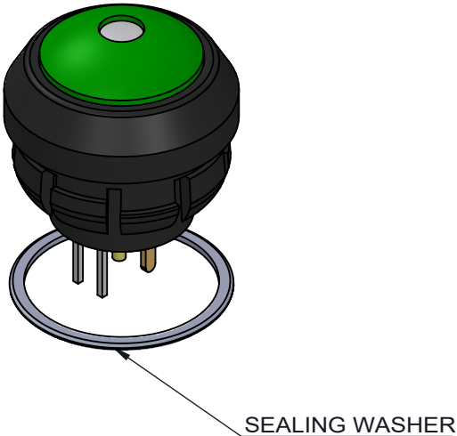
SNAP FIT TYPE
