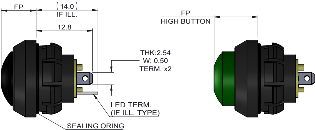
STANDARD BUTTON
