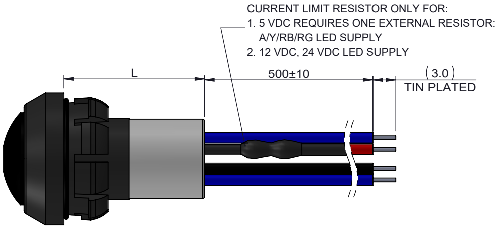
HIGH BUTTON
