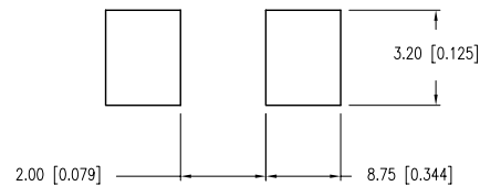
RECOMMENDED SOLDER PAD LAYOUT
