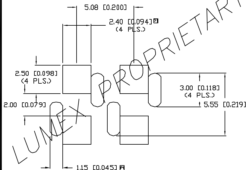
RECOMMENDED SOLDER PAD LAYOUT
