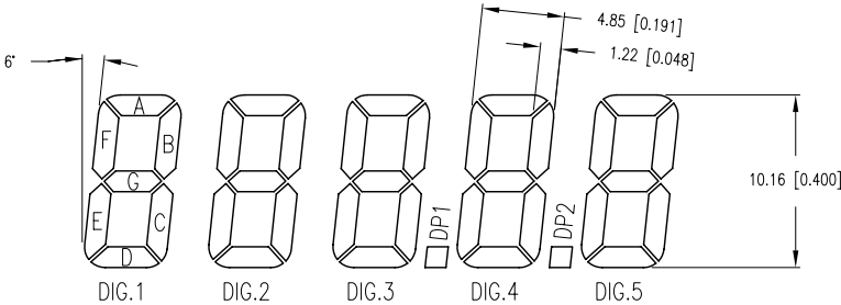
CHARACTER DETAIL
