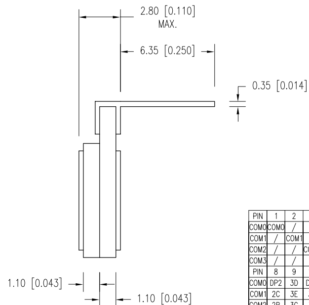
CHARACTERISTICS FLUID TYPE TN BACKGROUND COLOR GRAY VIEWING DIRECTION 6:00 DISPLAY MODE TRANSFLECTIVE OPERATING VOLTAGE 3.0V A.C. OPERATING TEMP. 0°C TO 50°C STORAGE TEMP. -20°C TO 70°C DRIVING METHOD 1/4 DUTY, 1/3 BIAS CONNECTION TYPE 13 PINS
