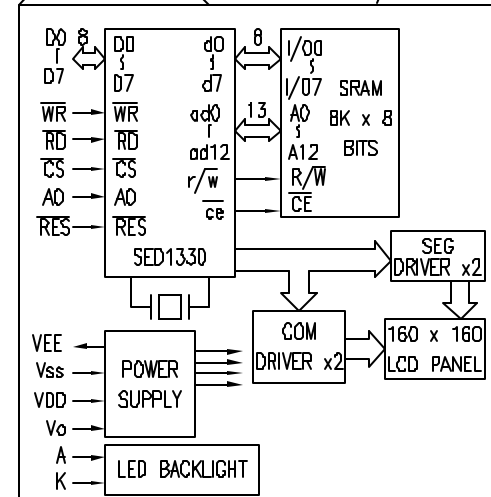
BLOCK DIAGRAM 160 x 160, 1/160 DUTY
