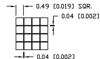
PIXEL DETAIL
