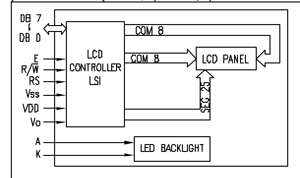
BLOCK DIAGRAM 10 x 1, 1/16 DUTY, 1/5 BIAS
