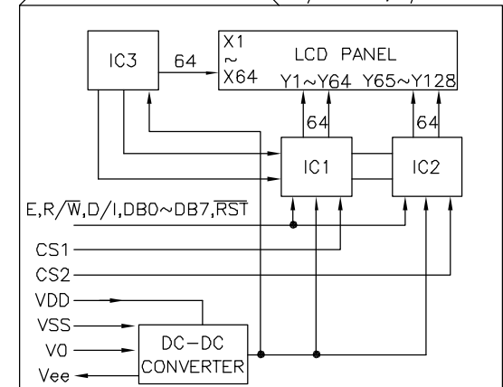
BLOCK DIAGRAM 1/64 DUTY, 1/6 BIAS
