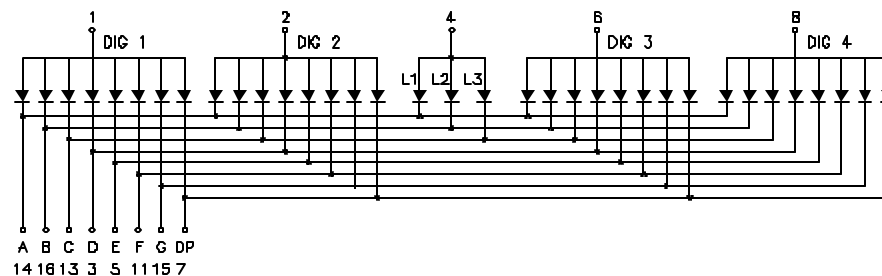
POLARITY DIAGRAM
