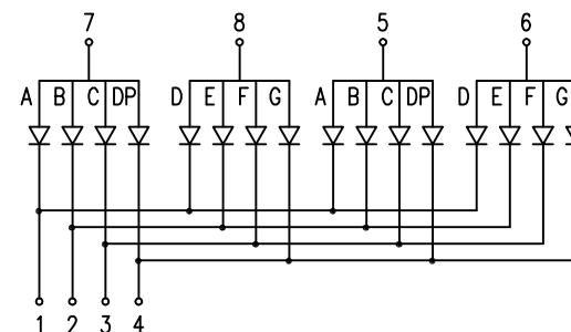
POLARITY DIAGRAM
