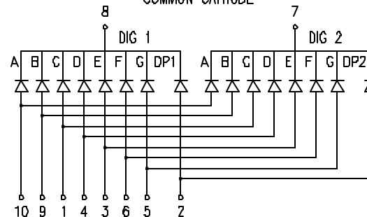
COMMON CATHODE
