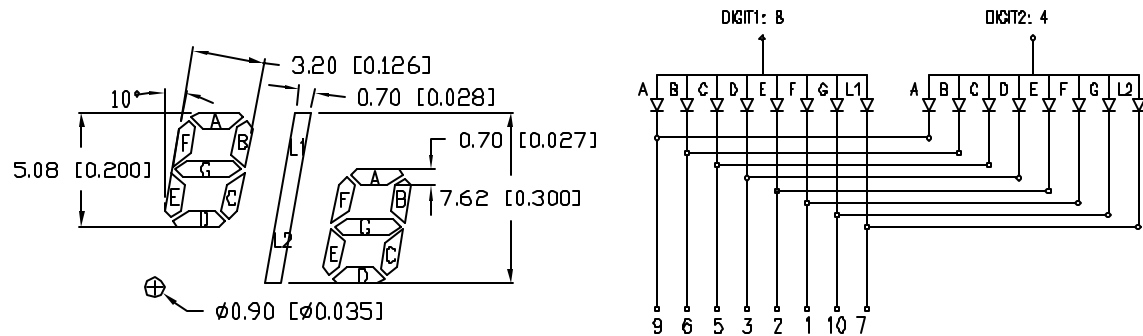
POLARITY DIAGRAM
