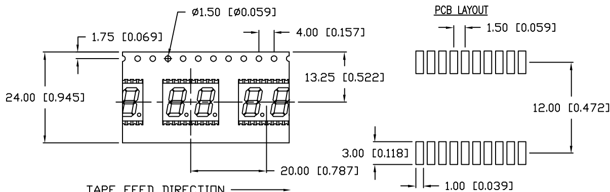
PCB LAYOUT
