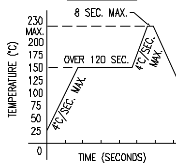
REFLOW PROFILE
