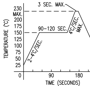
REFLOW PROFILE
