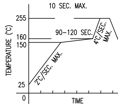
A LEAD FREE REFLOW PROFILE
