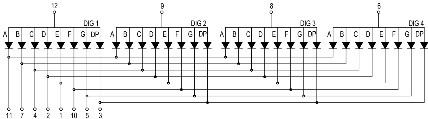
CIRCUIT DIAGRAM
