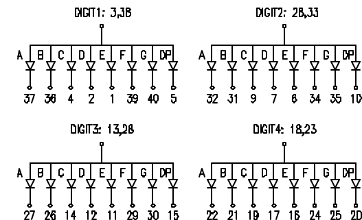
POLARITY DIAGRAM
