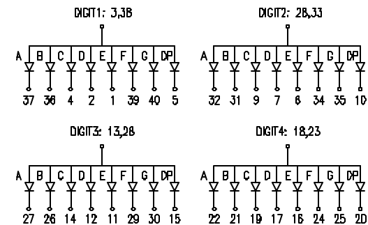
POLARITY DIAGRAM
