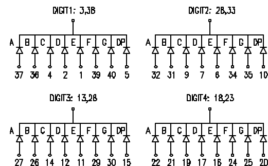
POLARITY DIAGRAM
