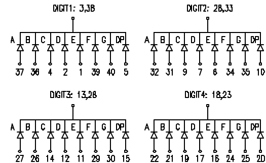
POLARITY DIAGRAM
