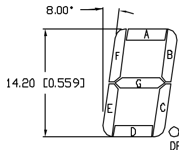
CHARACTER DETAIL
