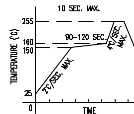
LEAD FREE REFLOW PROFILE
