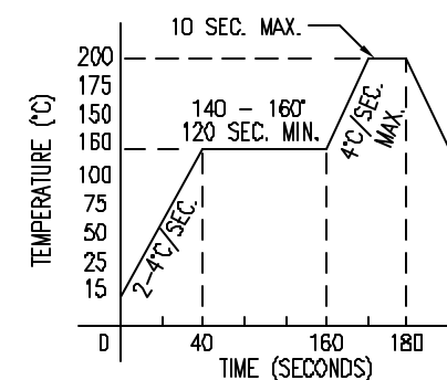
REFLOW PROFILE
