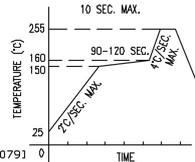
LEAD FREE REFLOW PROFILE
