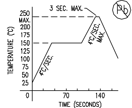
REFLOW PROFILE
