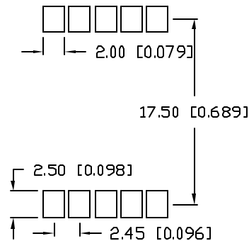
PCB LAYOUT
