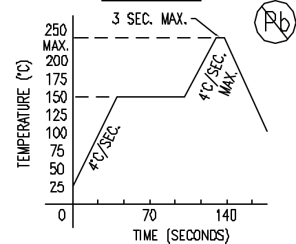
REFLOW PROFILE
