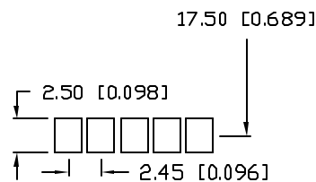
DETAIL SEGMENT VIEW
