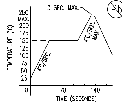
REFLOW PROFILE
