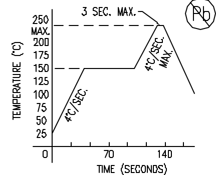
REFLOW PROFILE
