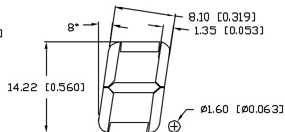
DETAIL SEGMENT VIEW
