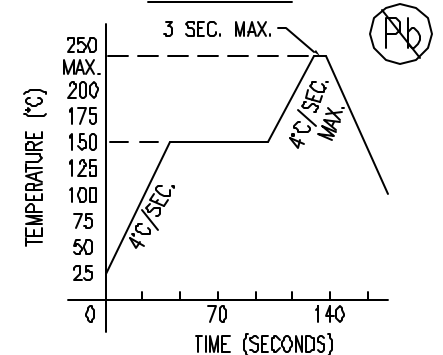
REFLOW PROFILE
