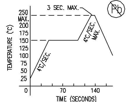
REFLOW PROFILE
