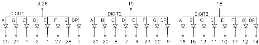
PIN LAYOUT
