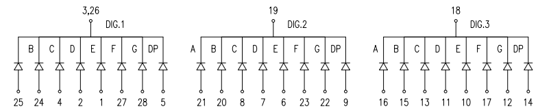
COMMON CATHODE
