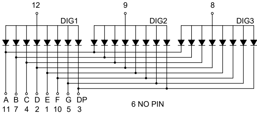
CIRCUIT DIAGRAM
