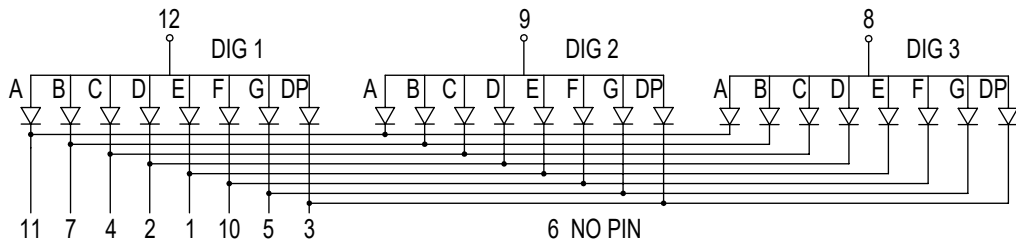
CIRCUIT DIAGRAM
