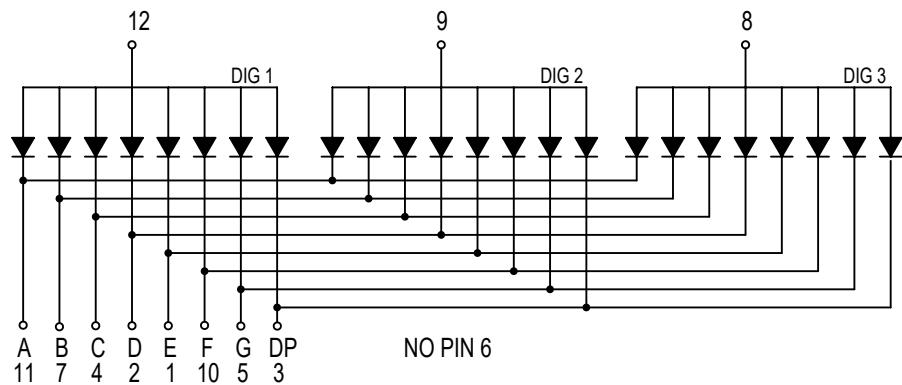
CIRCUIT DIAGRAM
