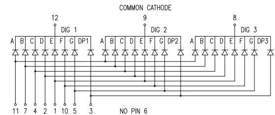
COMMON CATHODE
