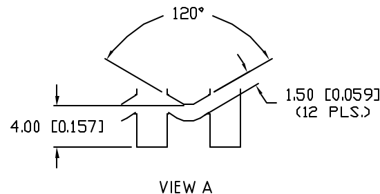
VIEW A
