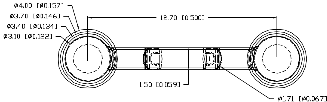
DETAIL A
