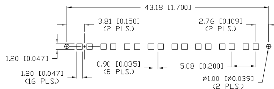
PCB LAYOUT
