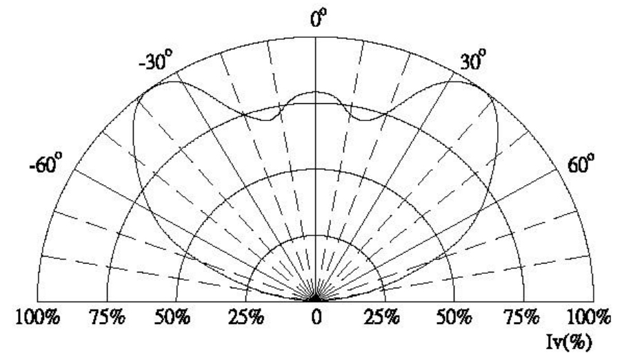
HORIZONTAL RADIATION CHARACTERISTIC
