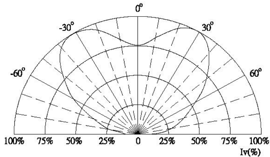
VERTICAL RADIATION CHARACTERISTIC
