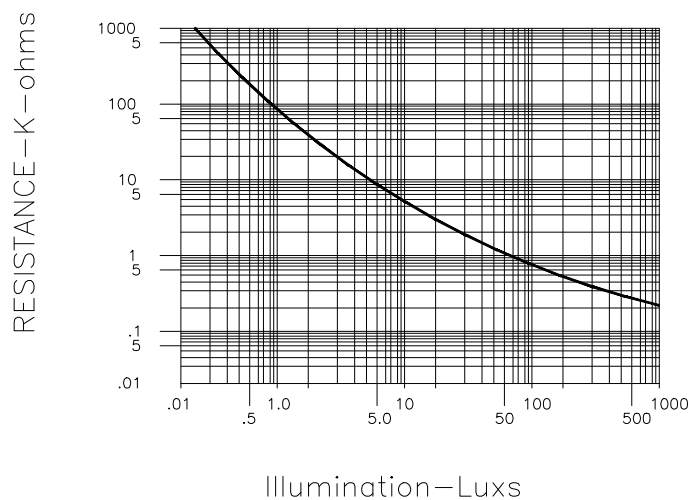
CELL RESISTANCE CURVES WITH VARIABLE ILLUMINATION
