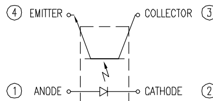
TOP VIEW PINLAYOUT
