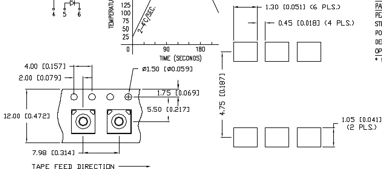
SOLDERING PAD LAYOUT
