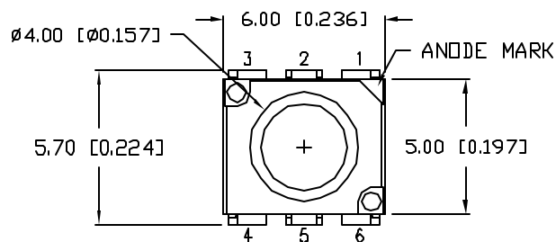
TOP VIEW POLARITY
