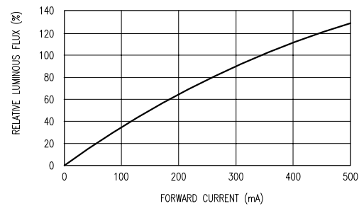
RELATIVE FLUX vs. CURRENT (Tj=25°C)
