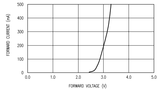
ELECTRICAL CHARACTERISTICS (Tj=25°C)
