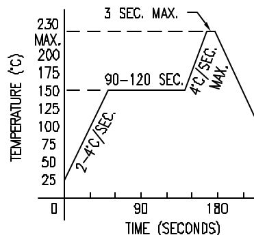
REFLOW PROFILE \Delta
