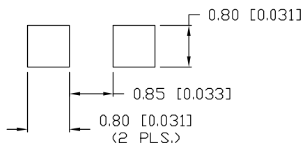
SOLDERING PATTERN
